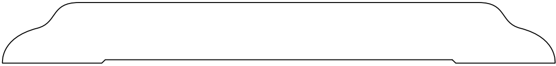
SAD6 5/8" x 5-5/8"
